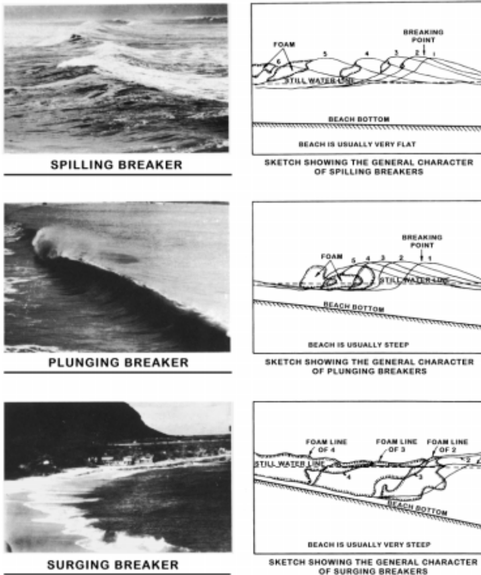
Figure 3317. The three types of breakers. Courtesy of Robert L. Wiegel, Council on Wave Research, University of California.
